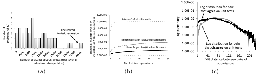
Fig. 5. (a) Histogram of the number of distinct abstract syntax trees (ASTs) submitted to each problem.; (b) Number of students covered by the 30 most common ASTs for several representative problems; (c) (Log) distribution over distances between pairs of submissions for pairs who agree on unit test outputs, and pairs who disagree. For very small edit distances ( <10 edits), we see that the corresponding submissions are typically also functionally similar (i.e., agree on unit test outputs).
