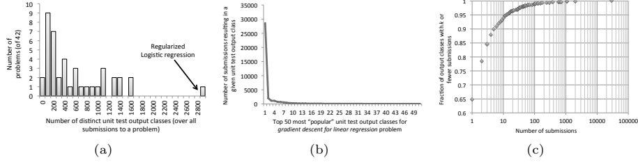
Fig. 3. (a) Histogram over the 42 problems of the number of distinct unit test outputs; (b) Number of submissions to each of the 50 most common unit test outputs for the “gradient descent for linear regression” problem; (c) Fraction of distinct unit test outputs with k or fewer submissions. For example, about 95% of unit test outputs owned fewer than 10 submissions.
